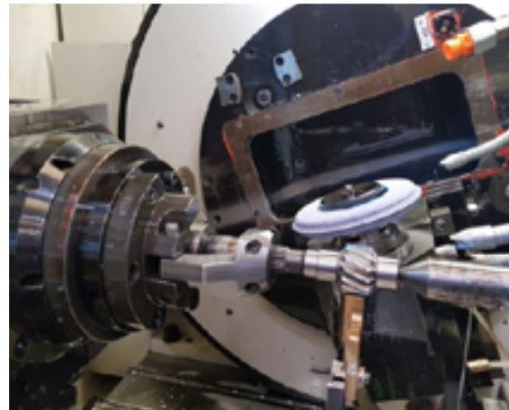
Samputensili S375
